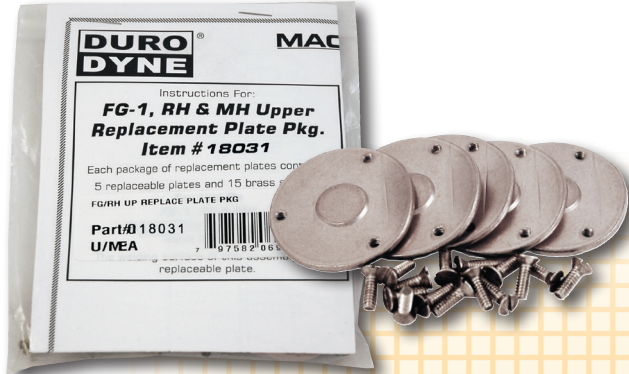
FG-1, RH & MH Upper Replacement Plate Pkg. Part# 18031 (replaces #17189)
