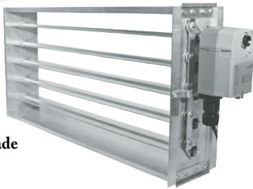
MMB Spring Return Mid-Torque Multi-Blade
